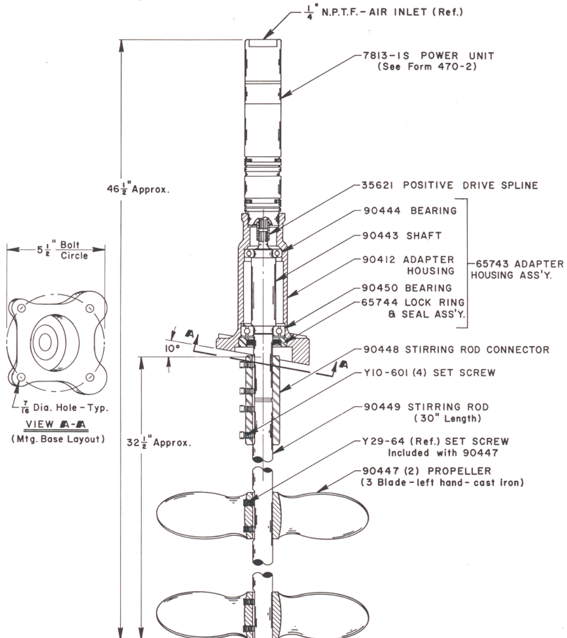
650251 MIXER MOTOR ASS'Y. (650 R.P.M. - .9 H.P.)
